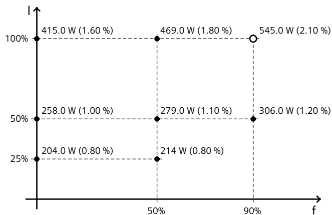
The percentage values show the losses in relation to the rated apparent power of the converter.
